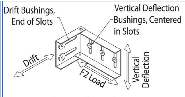
Fastener Pattern 2 replicates a condition of out-of-plane wind or seismic force with or without full vertical live load deflection and full in-plane drift.
