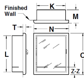
SEMI-RECESSED
