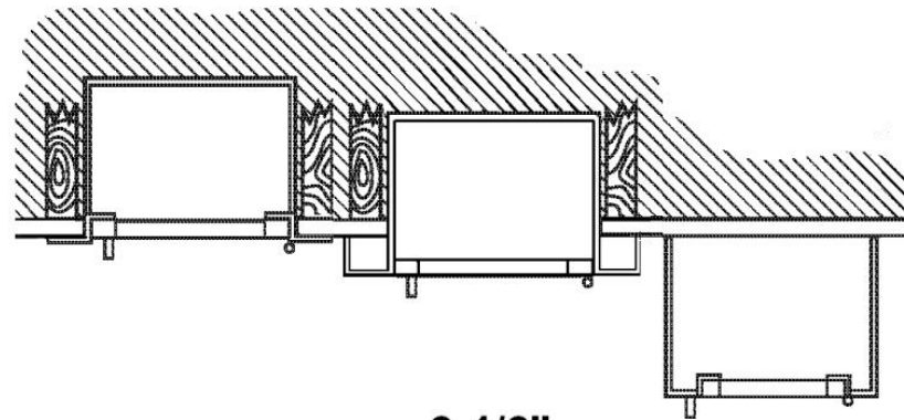
Flat Trim 2-1/2" Square Trim Square Edge Surface Mt.
